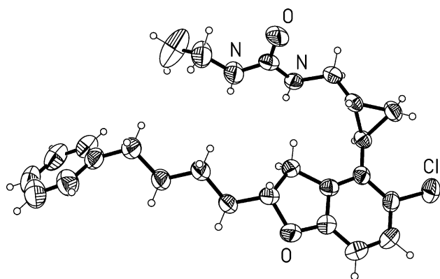
Figure 2. Thermal ellipsoid plot (35% ellipsoids) of crystalline 3g .
