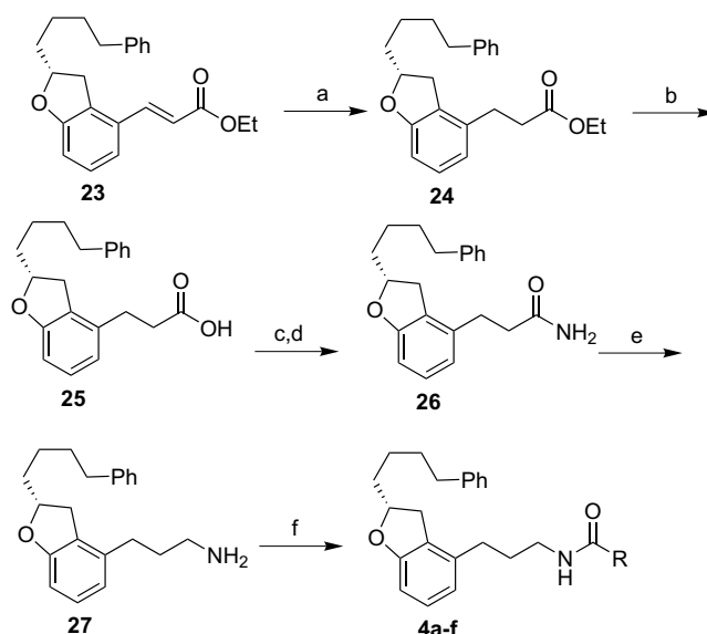
Scheme 2. Reagents and conditions: (a) \text{H}_2 , 10% Pd/C, AcOEt, rt, 100%; (b) NaOH, MeOH, reflux, 99%; (c) \text{SOCl}_2 , \text{CH}_2\text{Cl}_2 , reflux; (d) \text{NH}_3 , THF, -78 – -25 °C, 90% (two steps); (e) Red-Al, toluene, 0 – 25 °C, 94%; (f) \text{R}^1\text{COCl} , \text{Et}_3\text{N} , \text{CH}_2\text{Cl}_2 or \text{R}^2\text{NCO} , benzene.
