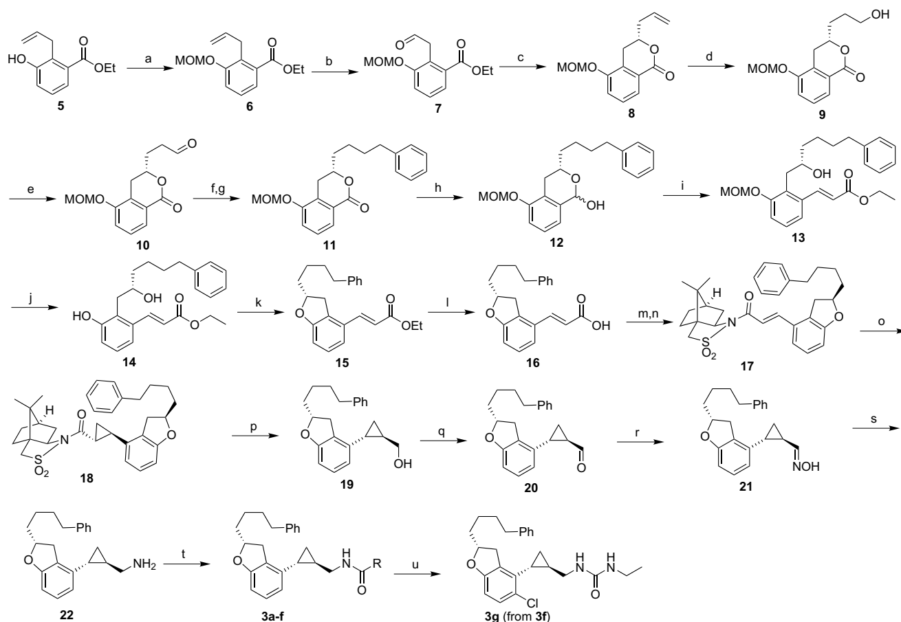
Scheme 1. Reagents and conditions: (a) MOMCl, i -Pr 2 NEt, CH 2 Cl 2 , rt, 96%; (b) OsO 4 , NaIO 4 , AcOEt, H 2 O, rt, 74%; (c) (–)- B -methoxydiisopinocampheylborane, allylmagnesium bromide, ether, 80%; (d) BH 3 ·THF, THF, H 2 O 2 , NaOH, 75%; (e) (COCl) 2 , DMSO, CH 2 Cl 2 , Et 3 N, 90%; (f) BnPPH 3 Br, n -BuLi, THF, 86%; (g) 10% Pd/C, H 2 , AcOEt, 99%; (h) DIBAL-H, PhMe, –78 °C, 99%; (i) Ph 3 PCHCO 2 Et, THF, reflux, 98%; (j) HCl, EtOH, rt, 100%; (k) Ph 3 P, DEAD, THF, 0–25 °C, 95%; (l) NaOH, MeOH, H 2 O, reflux, 96%; (m) SOCl 2 , CH 2 Cl 2 , reflux; (n) (1 S )-(–)-2,10-camphorsultam, NaH, PhMe, 0–25 °C, 92% (two steps); (o) CH 2 N 2 , Pd(OAc) 2 , CH 2 Cl 2 , 0–25 °C, 76%; (p) LAH, THF, 0–25 °C, 93%; (q) (COCl) 2 , DMSO, CH 2 Cl 2 , Et 3 N, –78–25 °C, 98%; (r) NH 2 OH·HCl, NaOH, THF, reflux, 98%; (s) LAH, reflux, 84%; (t) R 1 COCl, Et 3 N, CH 2 Cl 2 or R 2 NCO, benzene; (u) NCS, MeCN, reflux.
